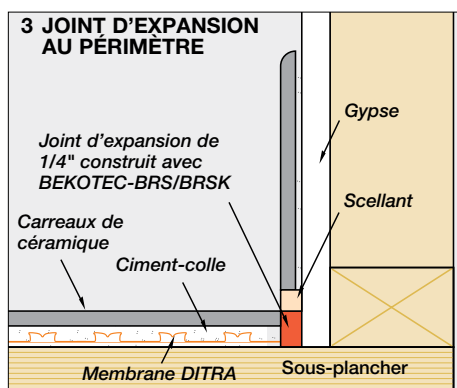
4 Schluter®-DILEX-BWS
