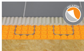
Schluter®- DITRA-HEAT-PS Page 120
