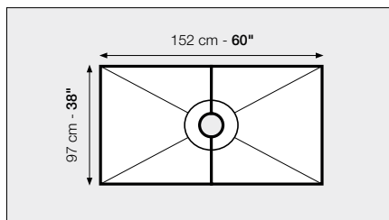
38" x 60" Kit - ABS or PVC
