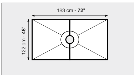
48" x 72" Kit - ABS or PVC
