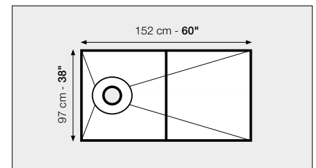
38" x 60" Kit off-center - ABS or PVC
