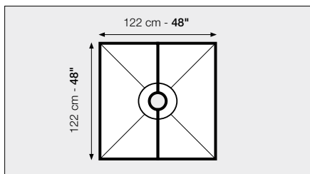
48" x 48" Kit - ABS or PVC
