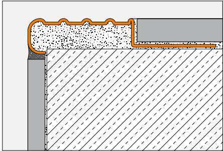
Installation variant for Schlüter®-TREP-E
