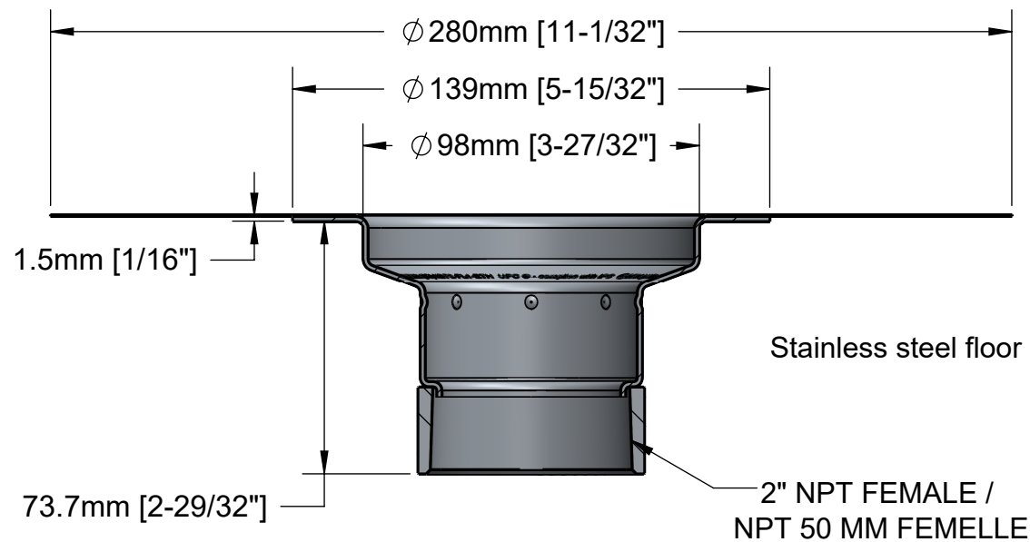
SECTION C-C
