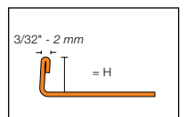
Multiple spacer design Stainless steel
