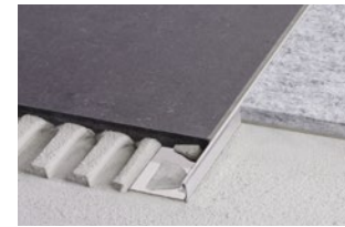
Schlüter®-SCHIENE-ES
