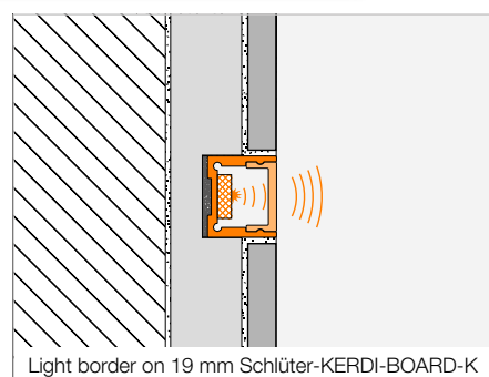
Light border on 19 mm Schlüter-KERDI-BOARD-K
