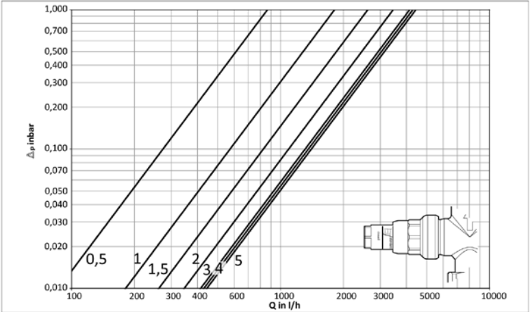
Figure 4: Balancing valve
