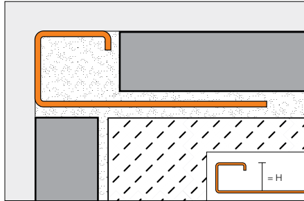
Inside/outside corner/end cap (EV/Q)
