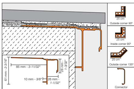
Outside corner 90°
