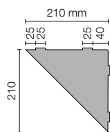
SHELF-E-S1
